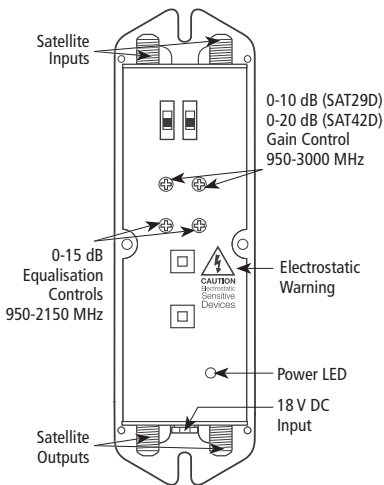
Fig. 1 (Lid removed)
